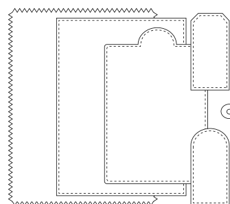
tag bundle die set pinked square 3 7/8 x 5 1/8", square tag 3 3/8 x 4 5/8" classic tag 2 5/8 x 4", small tags 1 x 2", hole 1/2 x 3/8" TAD0209 | set of 6 | $34.99
